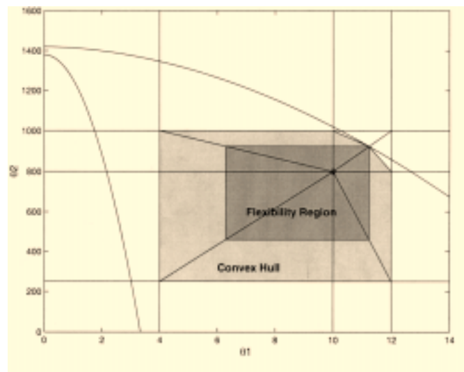
Figure 9. Example 2: feasible convex hull for design 1.
