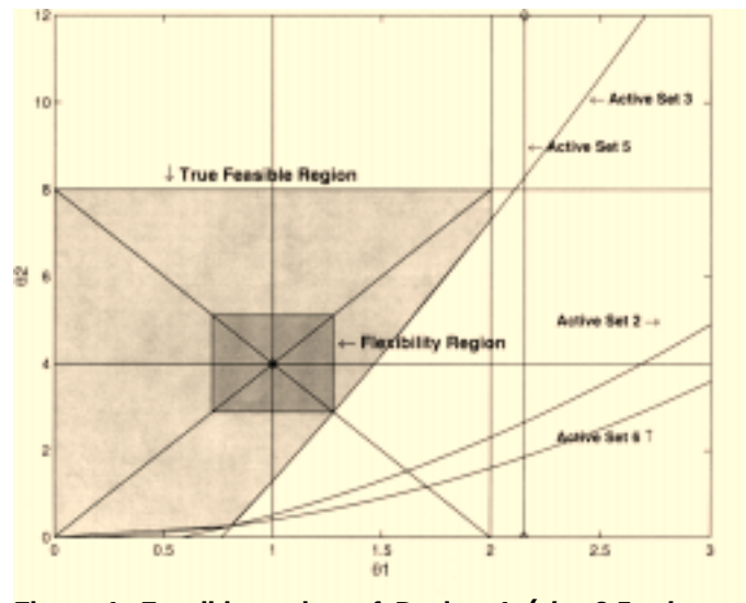
Figure 1. Feasible region of Design 1 ( d_1 = 3.5, d_2 = 0.0 ).
