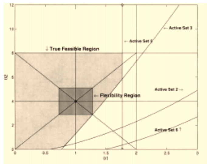
Figure 2. Feasible region of Design 2 ( d_1 = 2.5, d_2 = 3.5 ).
