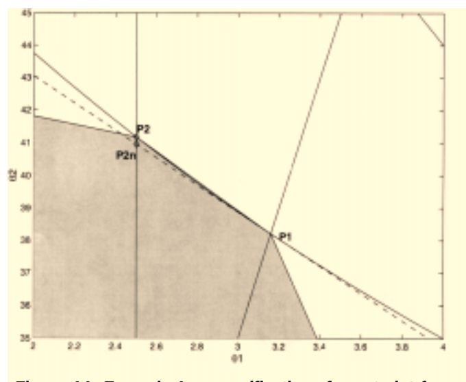
Figure 14. Example 4: convexification of constraint f_2 .
